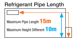
SRK10YL-S • SRK13YL-S SRK18YL-S
